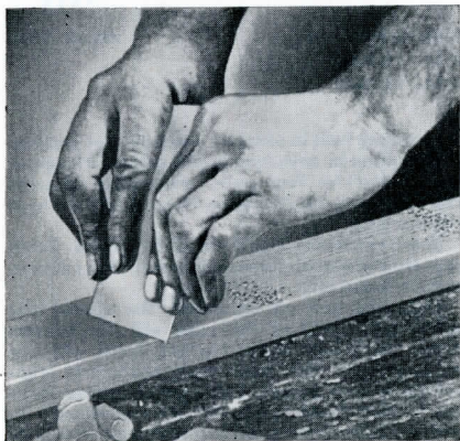
Proper way to hold cabinet scraper
