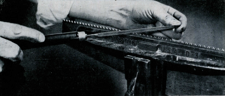
Position of file for beveling teeth
