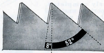
Side view of rip teeth (enlarged)
