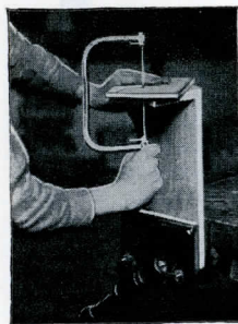
Using coping saw with saddle
