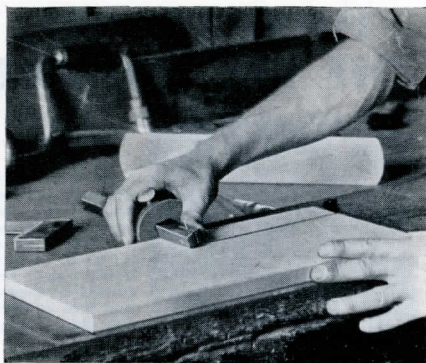
Scribing with a marking gauge
