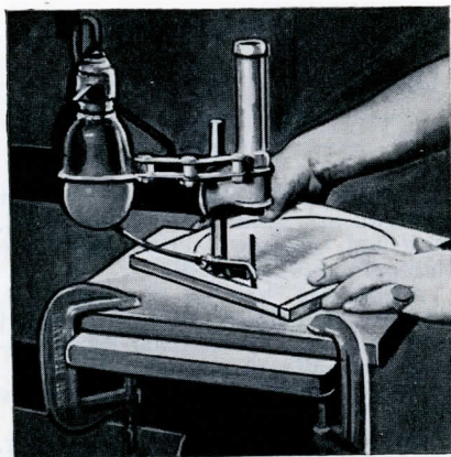
TO CUT circular discs on jig saw: clamp plywood board to table; use sharpened brad placed at one side of saw as center of disc. Pivot work on brad and revolve against saw.
