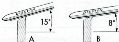
Turning the edge of a cabinet scraper, using a 4½-inch No. 1 Oval Burnisher.
