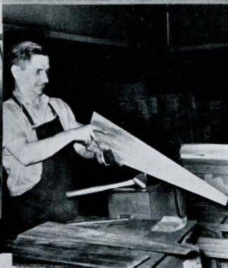
Hand saw smithing.
