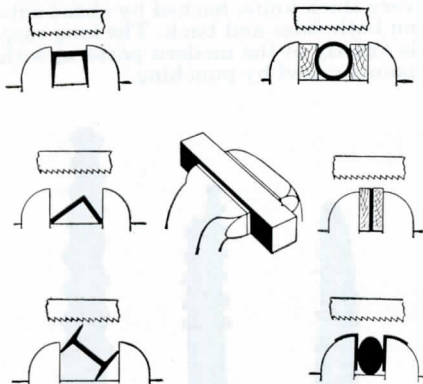
Two teeth and more on section
